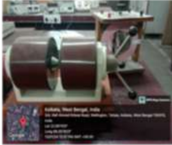
Gouy's balance set up
